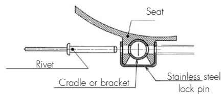
PRINCIPLE OF CLIPPING AND LOCKING ON REAR CLAMPS
